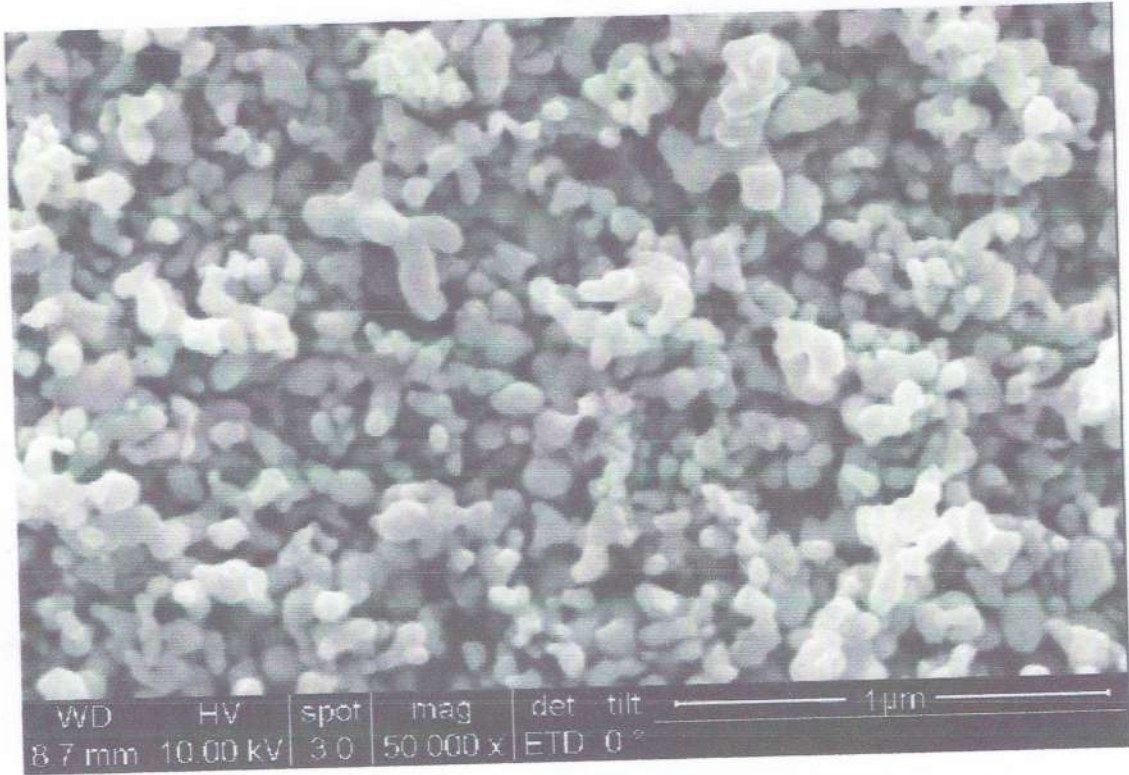
SEM Image of Nano Silver 80 nm
