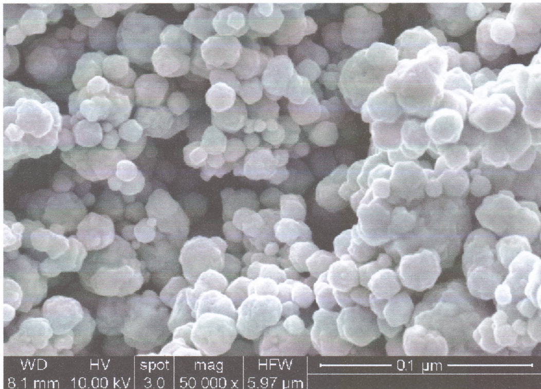
SEM Image of Nano Silver 20 nm
