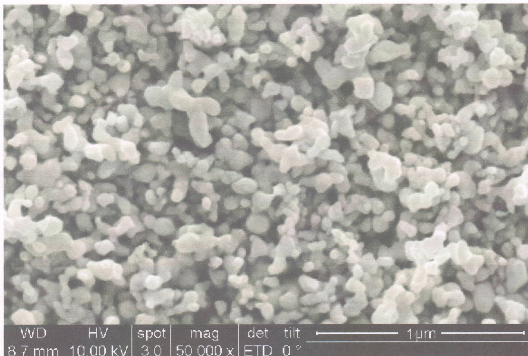
SEM Image of Nano Silver 80 nm
